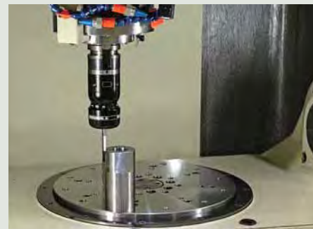
Measurement of C axis rotation center
